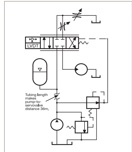
Fig. 3 Test circuit to generate and measure shock waves in a hydraulic system
